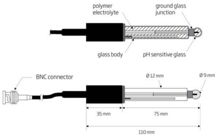
Combination Glass-body pH Electrode
