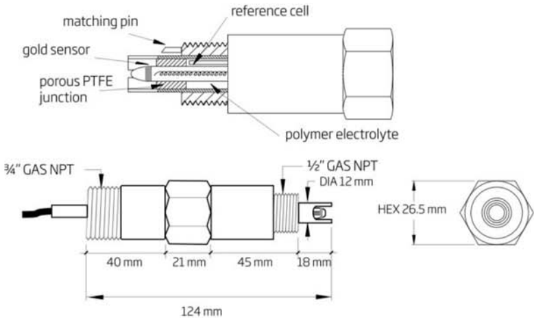
HI2000 Series: ORP Electrodes with Gold Sensor
