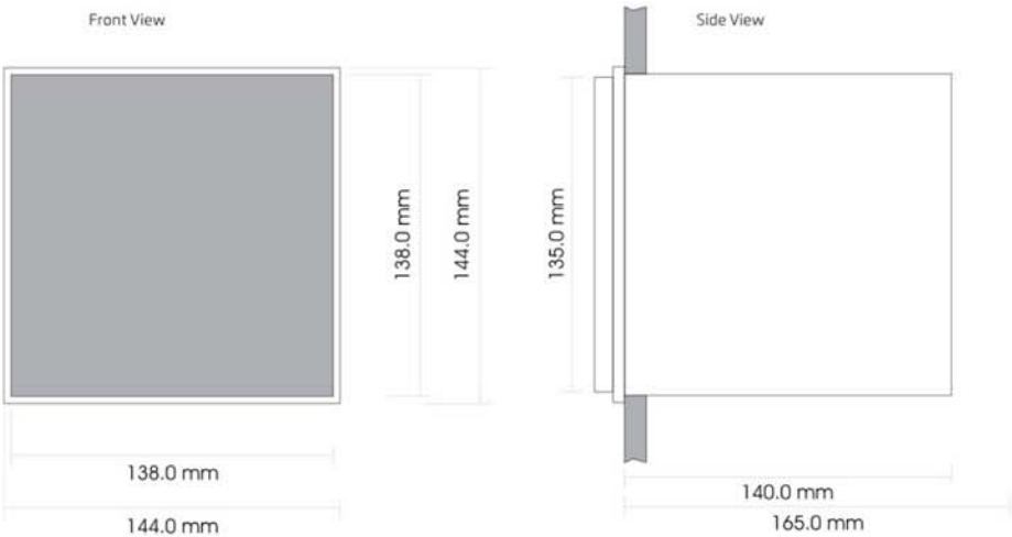
Mechanical Dimensions
