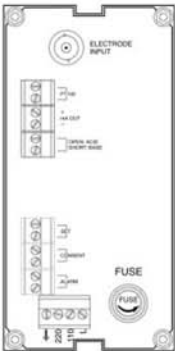
Rear View Rear view of the HI8710 shows the typical electrical connections.
