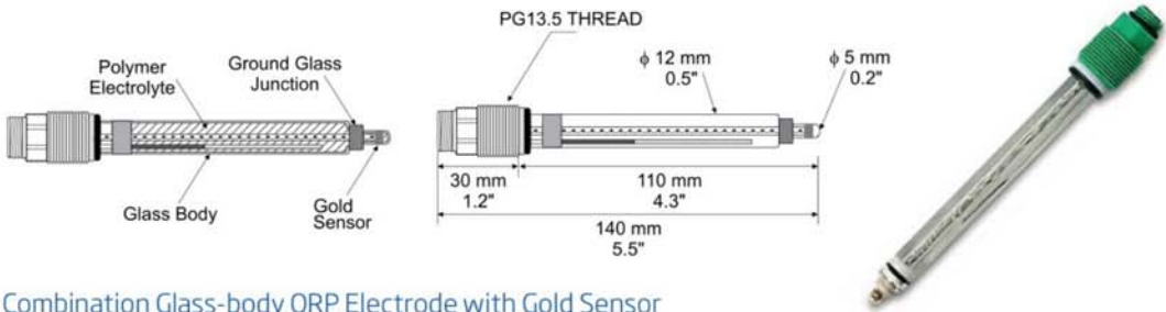
Combination Glass-body ORP Electrode with Gold Sensor
